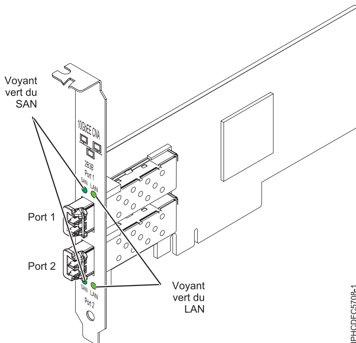
Figure 30. carte PCIe LP 10 gigabits FCoE 2 ports
