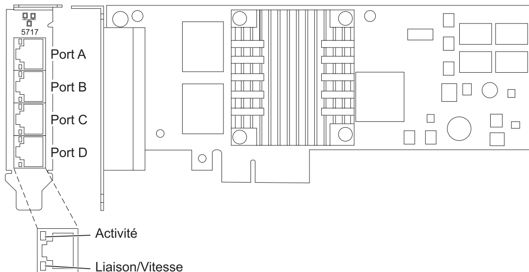
Figure 44. Carte PCIe 10/100/1000 Base-TX 4 ports
