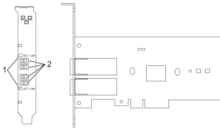
Figure 33. carte PCIe LP 2 ports 1GbE SX
