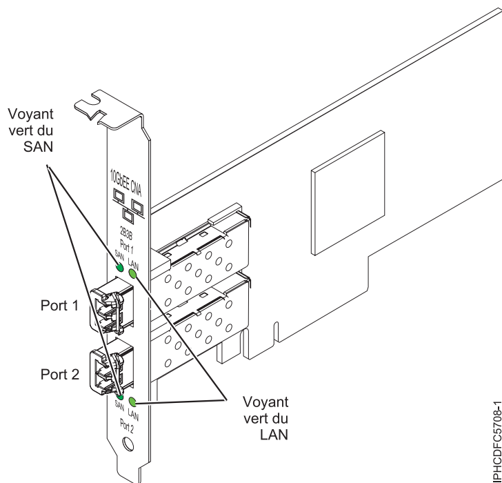
Figure 43. carte double port PCIe FCoE 10 Gb
