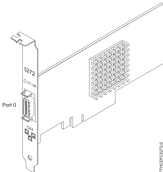
Figure 32. carte PCIe LP 10GbE CX4 1 port
