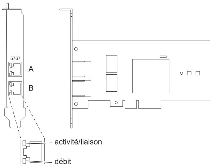
Figure 51. Carte PCI Express Ethernet 10/100/1000 Base-TX 2 ports
