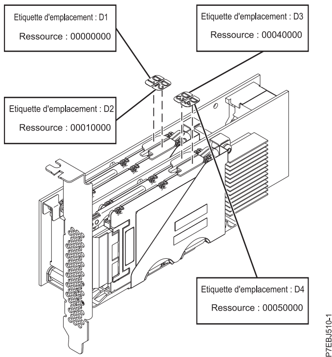
Figure 64. Carte SAS RAID PCIe Dual - x4 3 gigabits
