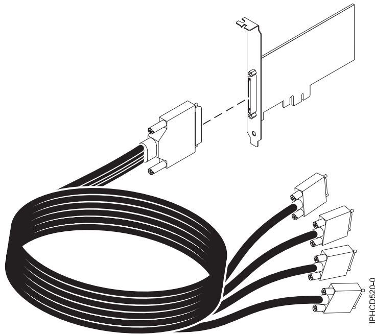
Figure 6. Câble
