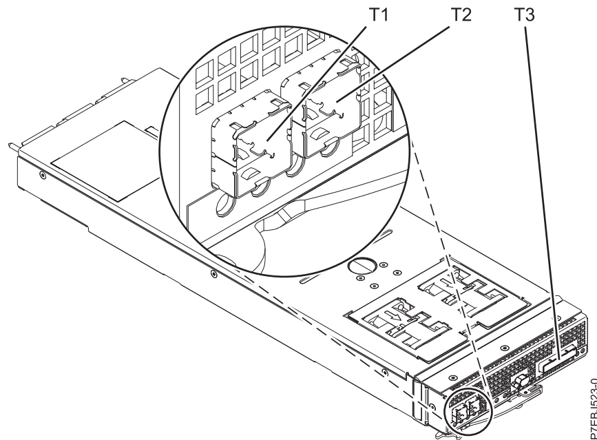
Figure 85. CCIN 57C3 - Boîtier SAS RAID cache PCIe2 3,1 Go 6 gigabits x8.
