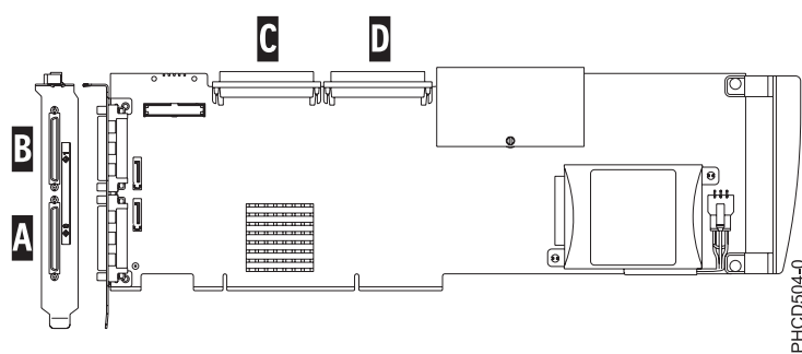
Figure 77. Carte RAID SCSI PCI-X DDR double canal Ultra320
