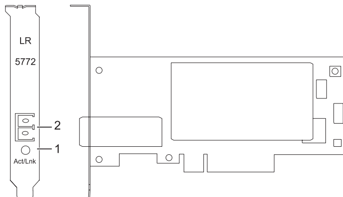
Figure 54. Carte PCI Express Ethernet-LR 10 gigabits
