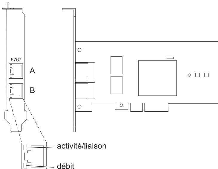
Figure 56. carte PCIe 2 ports 1GbE TX
