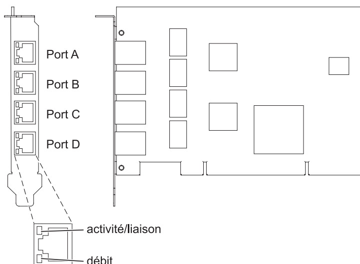
Figure 47. Carte PCI-X 4 ports 10/100/1000 Base-TX
