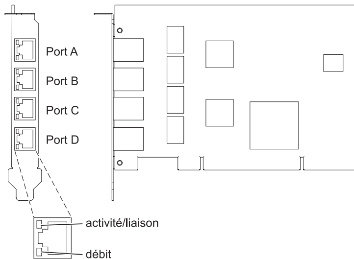
Figure 46. Carte PCI-X 4 ports 10/100/1000 Base-TX
