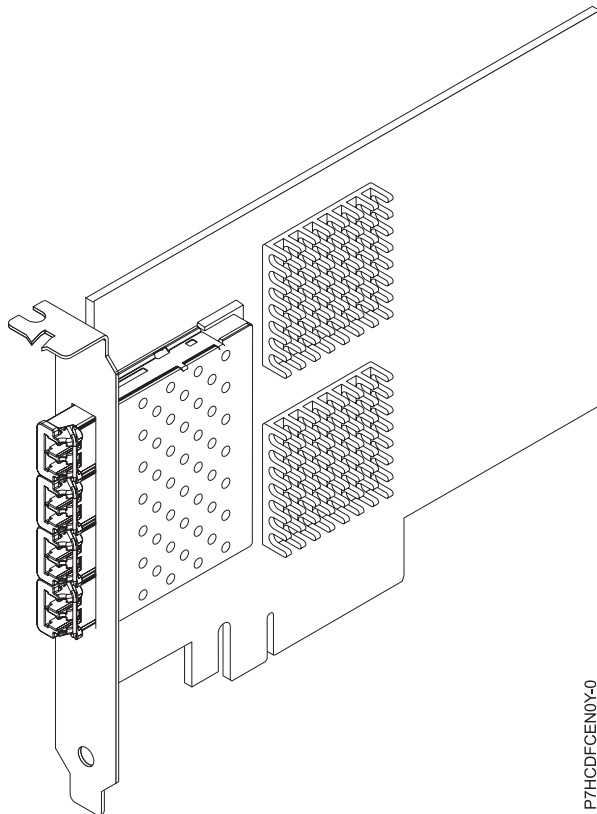
Figure 21. carte Fibre Channel PCIe2 4 ports 8 gigabits LP
