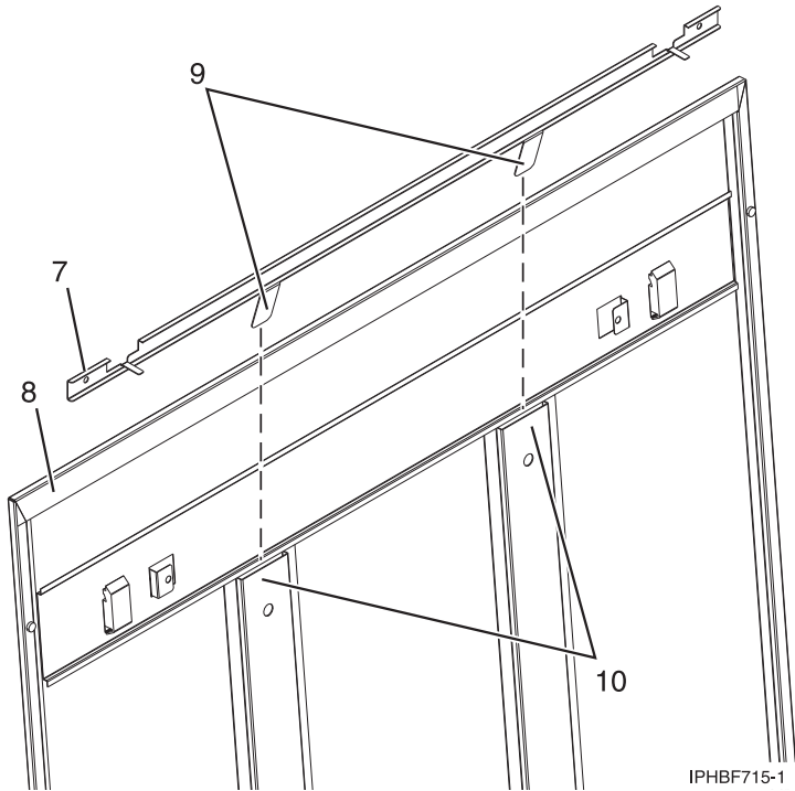
Figure 77. Installing a security slide bar
