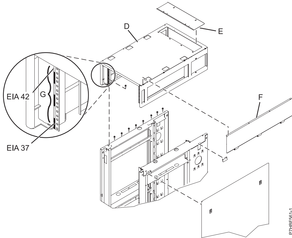
Figure 92. Removing the top cover
