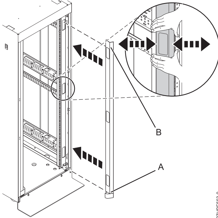
Figure 72. Installing the rack trim panel
