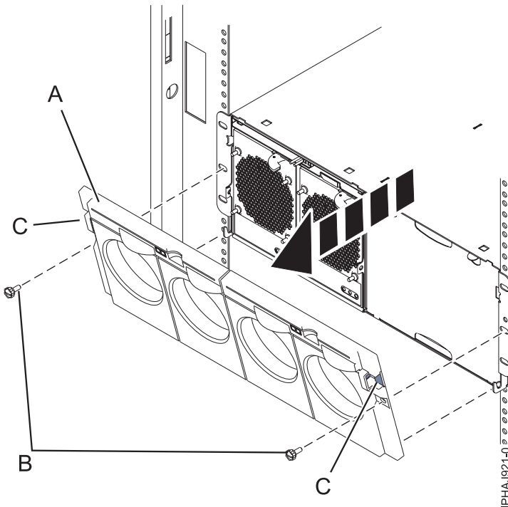
Figure 100. Remove the front cover for model 7314-G30 or 5796
