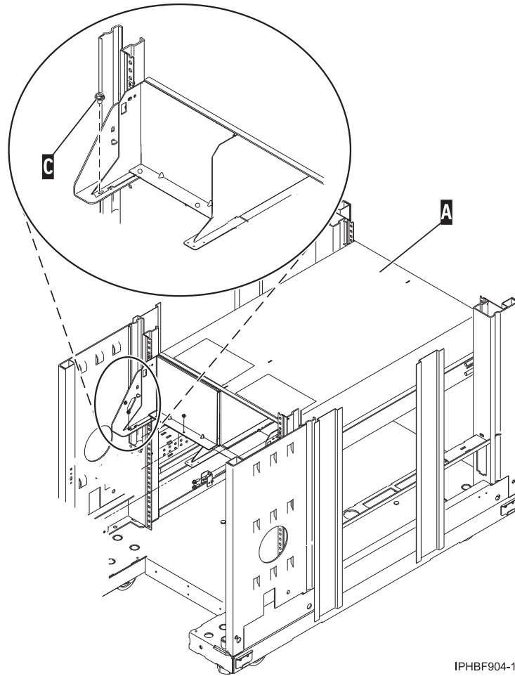
Figure 57. Securing the shell to the rack with the expandable rails
