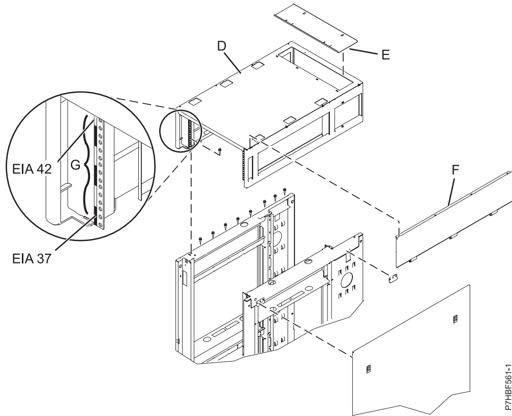
Figure 91. Removing the top cover
