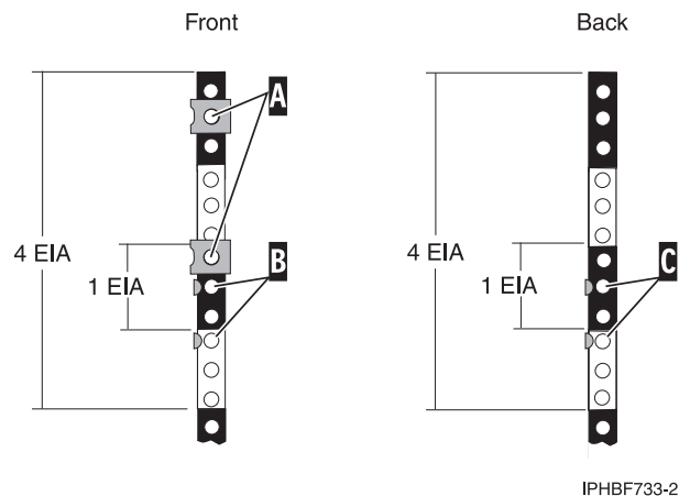
Figure 61. Marking the installation locations
