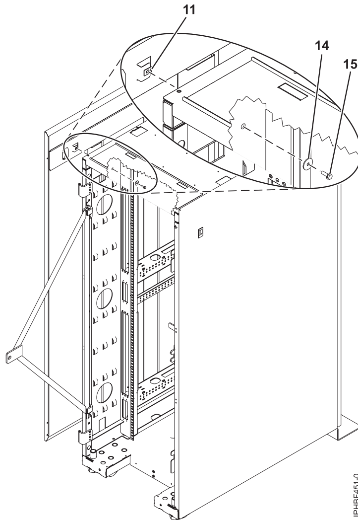
Figure 81. Removing the securing screws on the side panel
