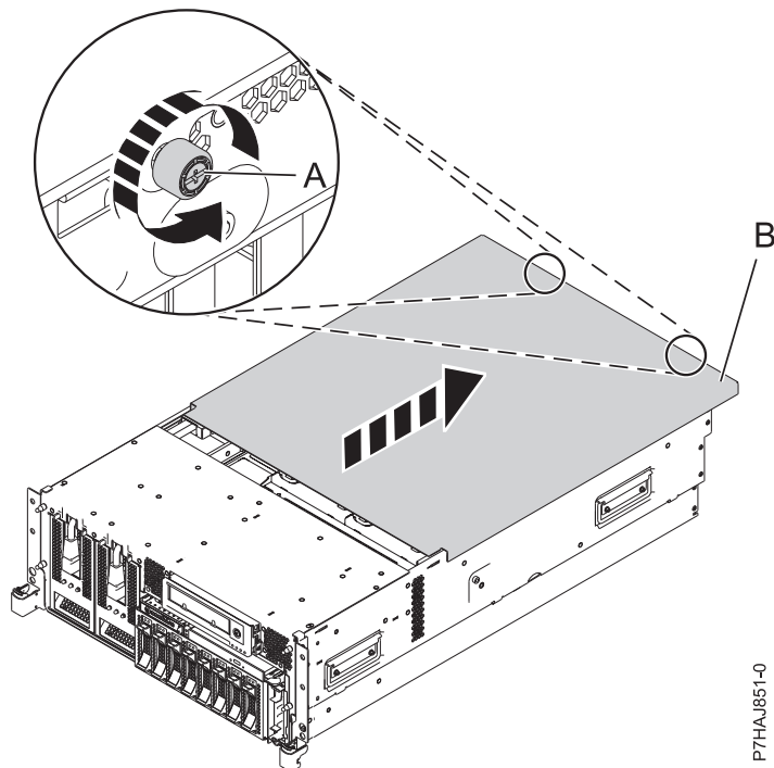
Figure 102. Removing the service access cover
