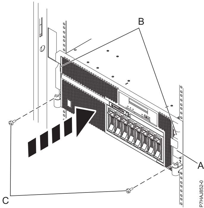
Figure 105. Installing the front cover
