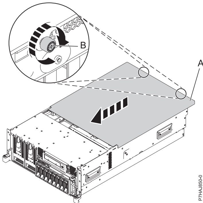
Figure 103. Installing the service access cover
