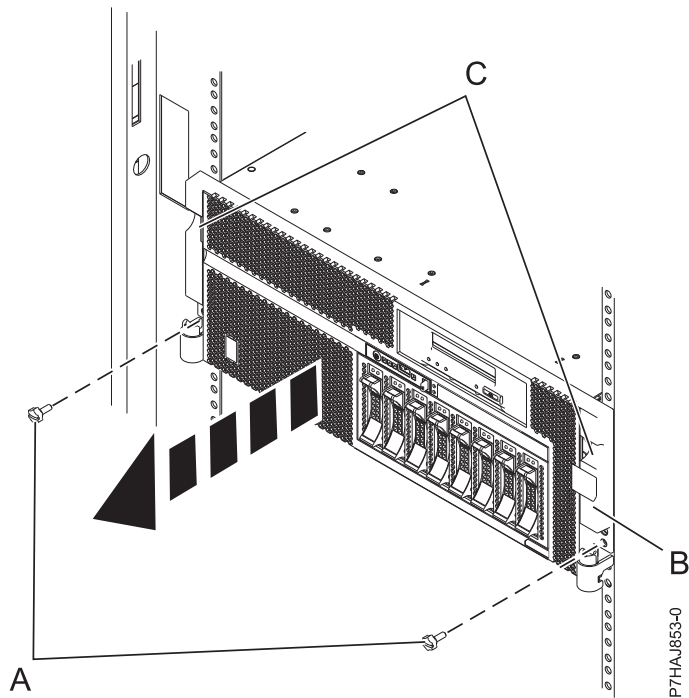
Figure 104. Removing the front cover
