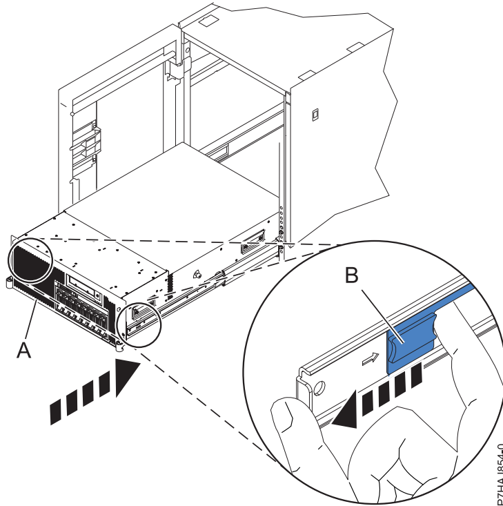
Figure 112. Releasing the rail safety latches
