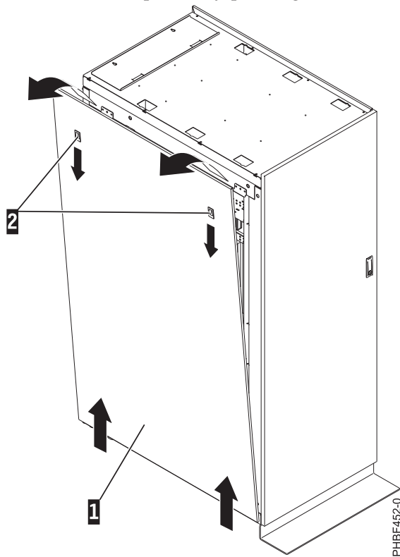
Figure 69. Removing the side panel
