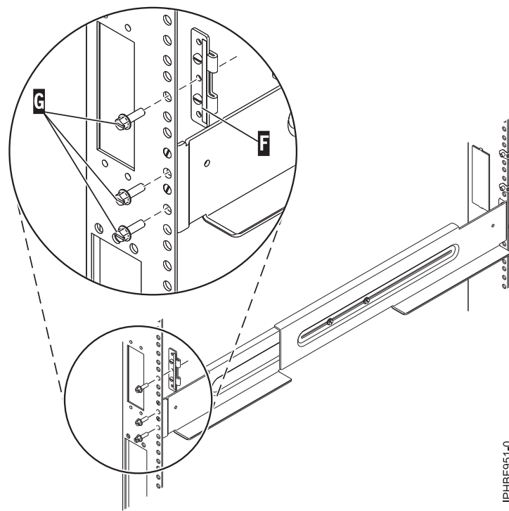
Figure 55. Attaching the rails to the back of the rack
