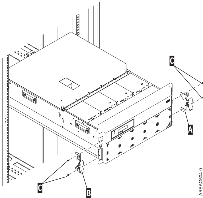
Figure 88. Reinstalling the latch brackets
