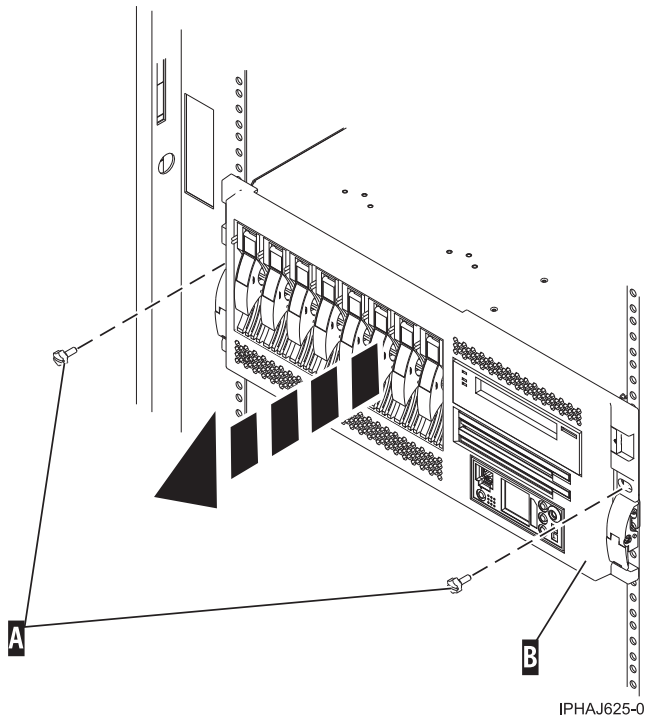
Figure 107. Removing the screws from the system and rack
