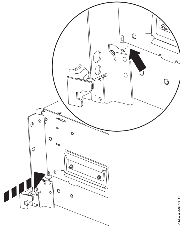
Figure 25. Align the bracket with the slot on the side of the system
