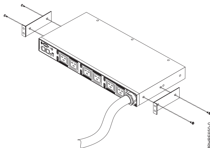
Figure 97. Aligning the vertical-mounting brackets to the front of the PDU+.
