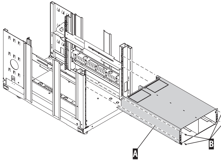
Figure 56. Installing the shell into the rack on the expandable rails
