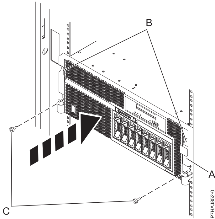
Figure 110. Pushing the system into the rack and attaching the screws
