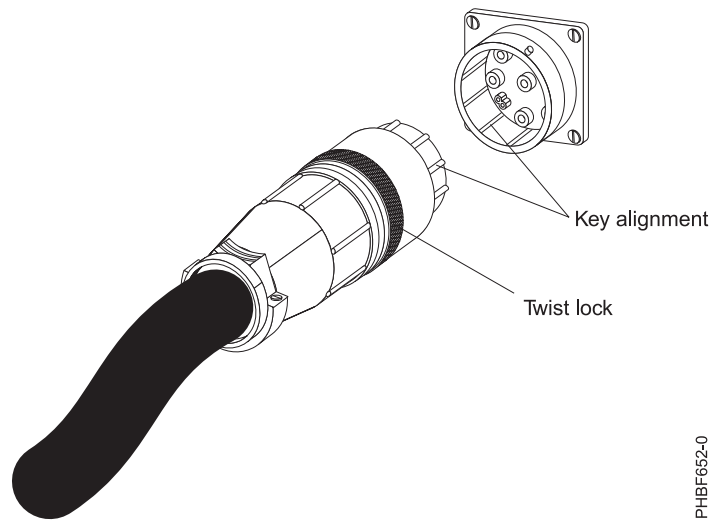
Figure 96. Aligning the connector on the power cord with the PDU+
