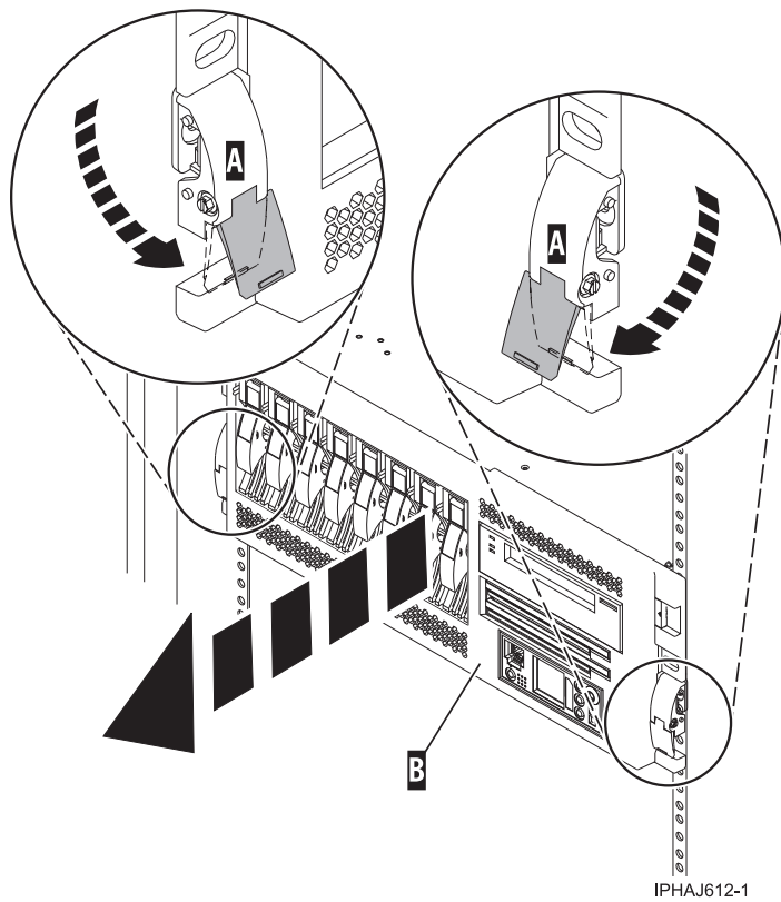
Figure 108. Releasing the rack latches
