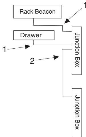
Figure 87. Connect the rack status beacon and system unit to the junction box
