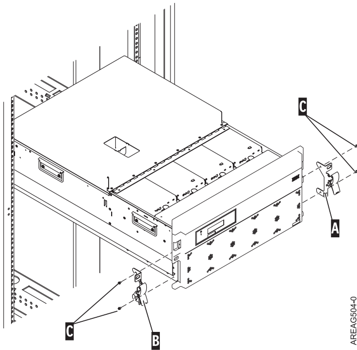
Figure 89. Removing the retaining screws
