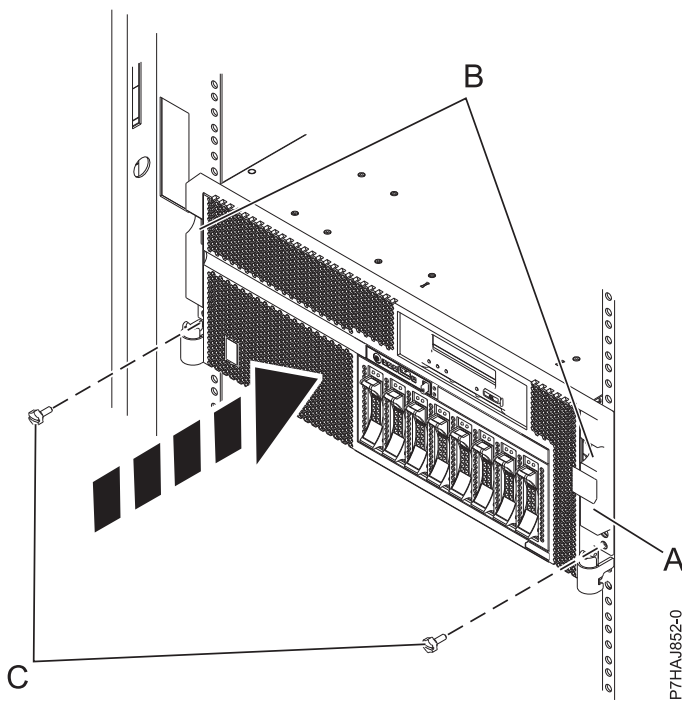
Figure 113. Replacing the thumbscrews
