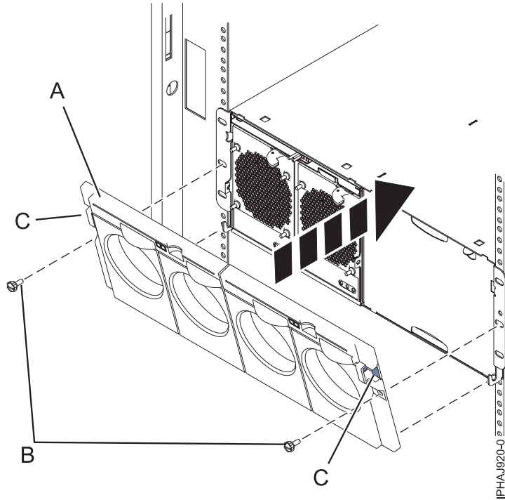
Figure 101. Front cover on a model 7314-G30 or 5796
