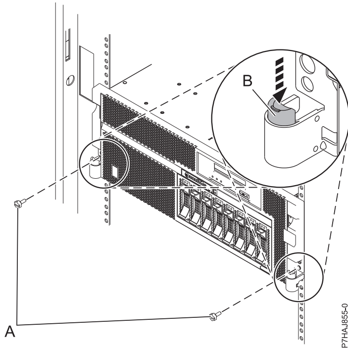
Figure 111. Releasing the rack latches
