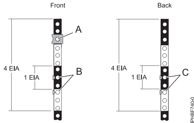
Figure 34. Marking the installation locations
