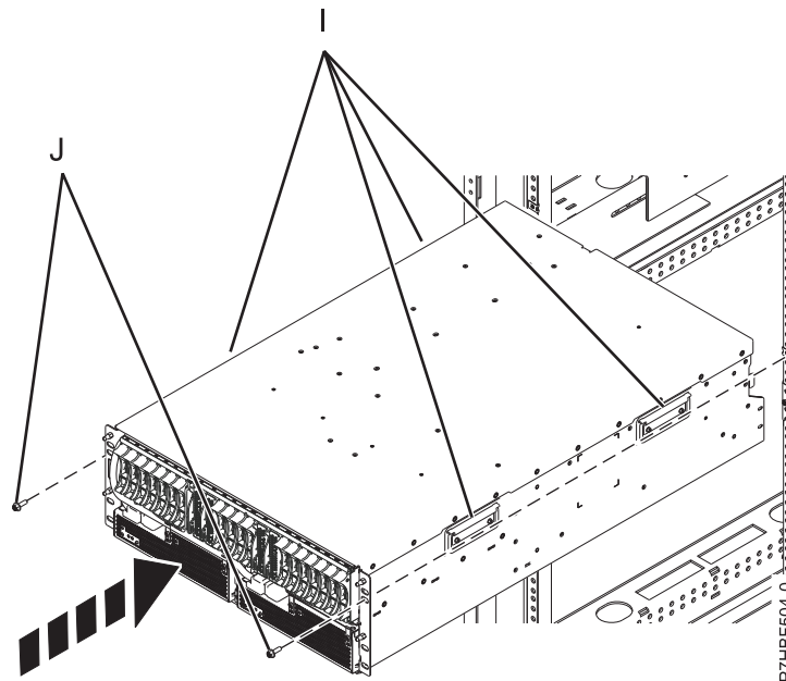
Figure 39. Installing the expansion unit into a rack
