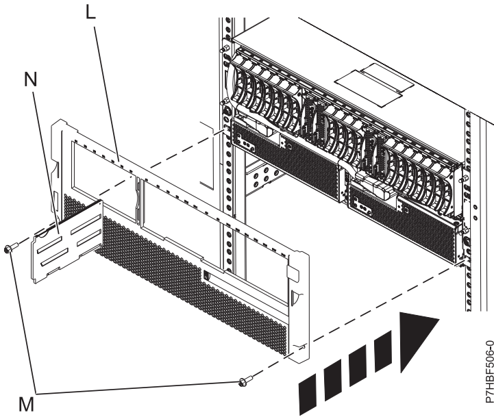
Figure 40. Installing the bezel and service information holder
