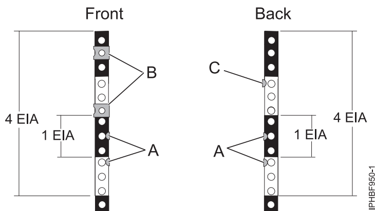
Figure 52. EIA units with expandable rails for the 5796 expansion unit
