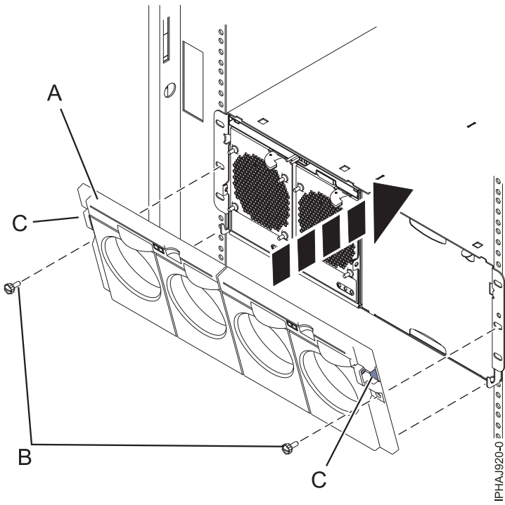
Figure 106. Front cover on a model 7314-G30 or 5796
