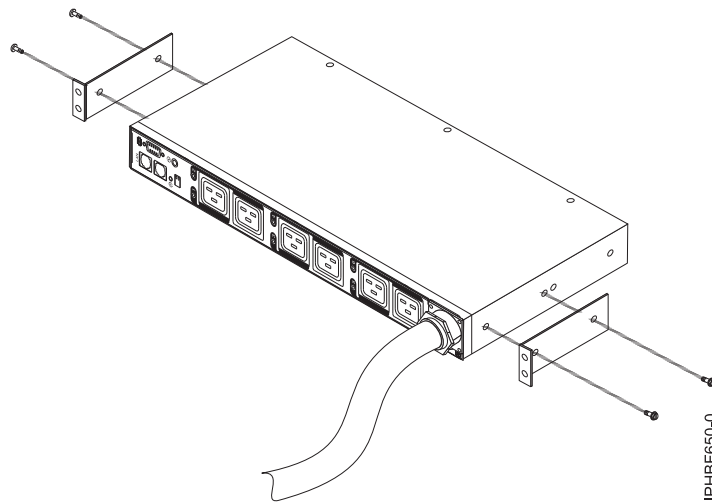
Figure 94. Aligning the vertical-mounting brackets to the front of the PDU+
