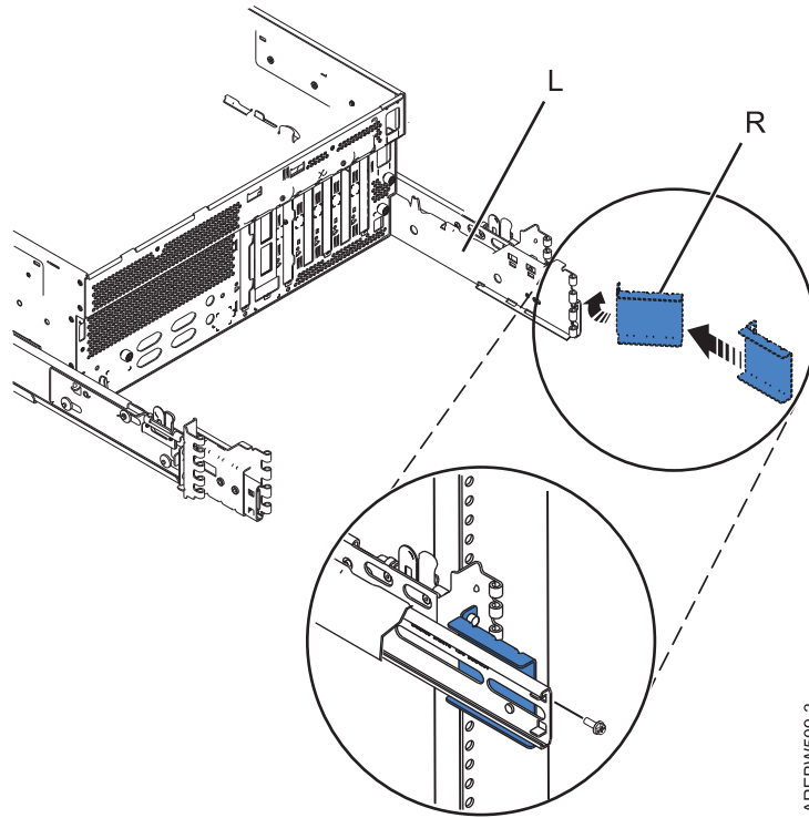
Figure 23. Installing the rail support brackets
