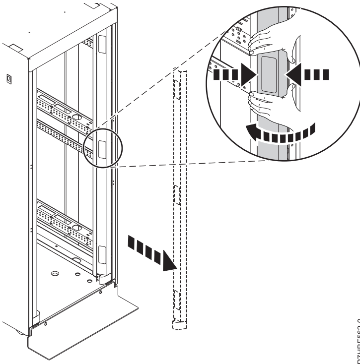
Figure 71. Removing the rack trim panel
