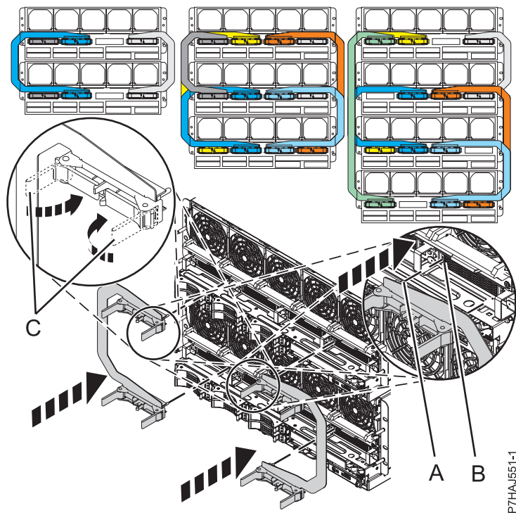
Figure 13. Installation du câble SMP
