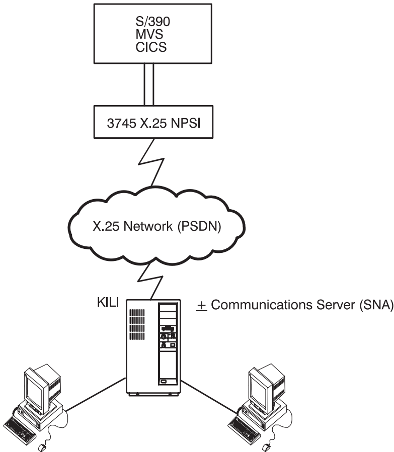
Figure 11. Example of a SNA Connection Using X.25. An X.25 network (PSDN) being used to provide communication between (a) an RS/6000® or eServer pSeries® system running SNA services with X.25 and (b) a System 390 or eServer zSeries host.
