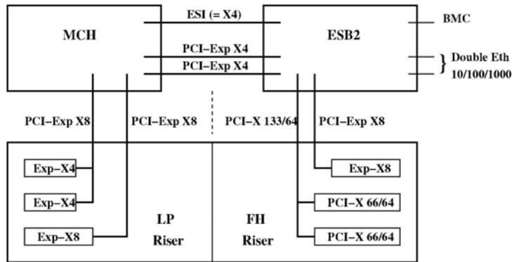
Figure F-5. R460 risers and I/O subsystem slotting
