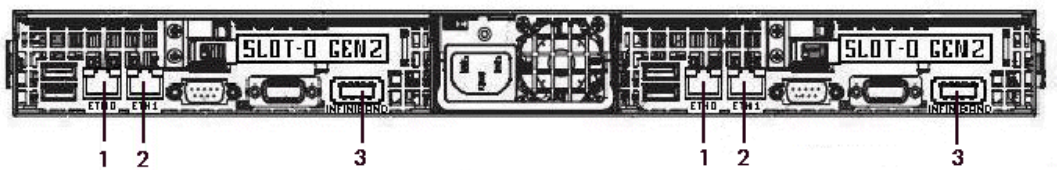
Figure F-9. Rear view of R422 E1 Series (2 Compute Nodes in 1U with Integrated InfiniBand)
