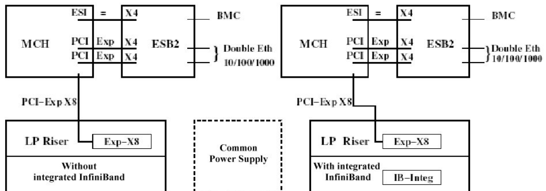
Figure F-3. R422 rear view of Riser architecture
