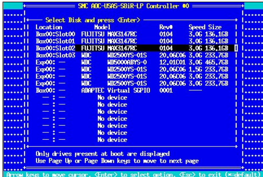
Figure E-16. An example of a drive list for an Adaptec controller
