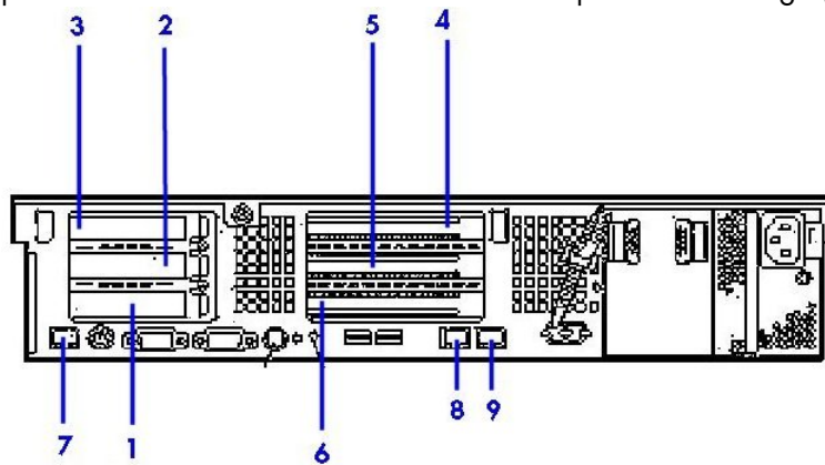
Figure F-6. Rear view of R460 Series
