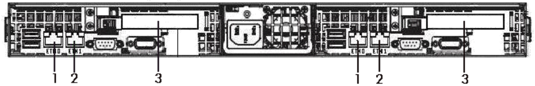
Figure F-8. Rear view of R422 E1 Series (2 Compute Nodes in 1U)
