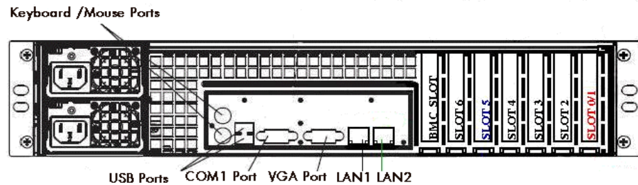
Figure F-11. Rear view of R423 E1 Series
