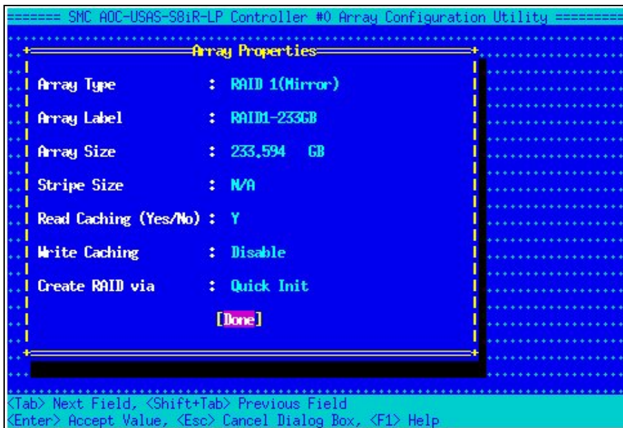
Figure E-10. Array Properties - Confirmation screen
