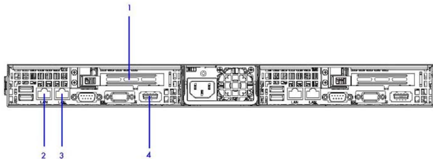
Figure F-4. R422 Rear view connectors
