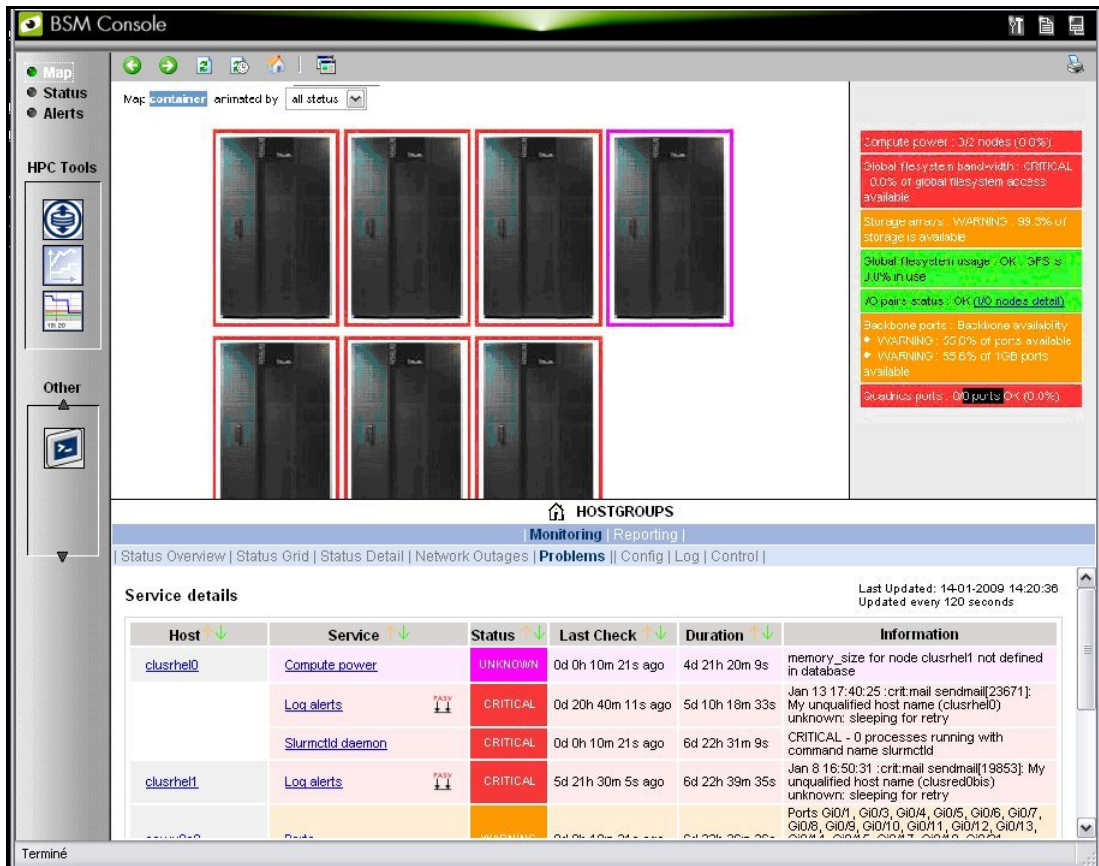
Figure 3-24. Bull System Manager Monitoring Window
