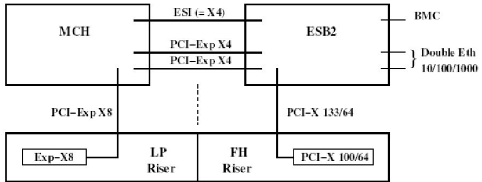
Figure F-1. R421 rear view of Riser architecture
