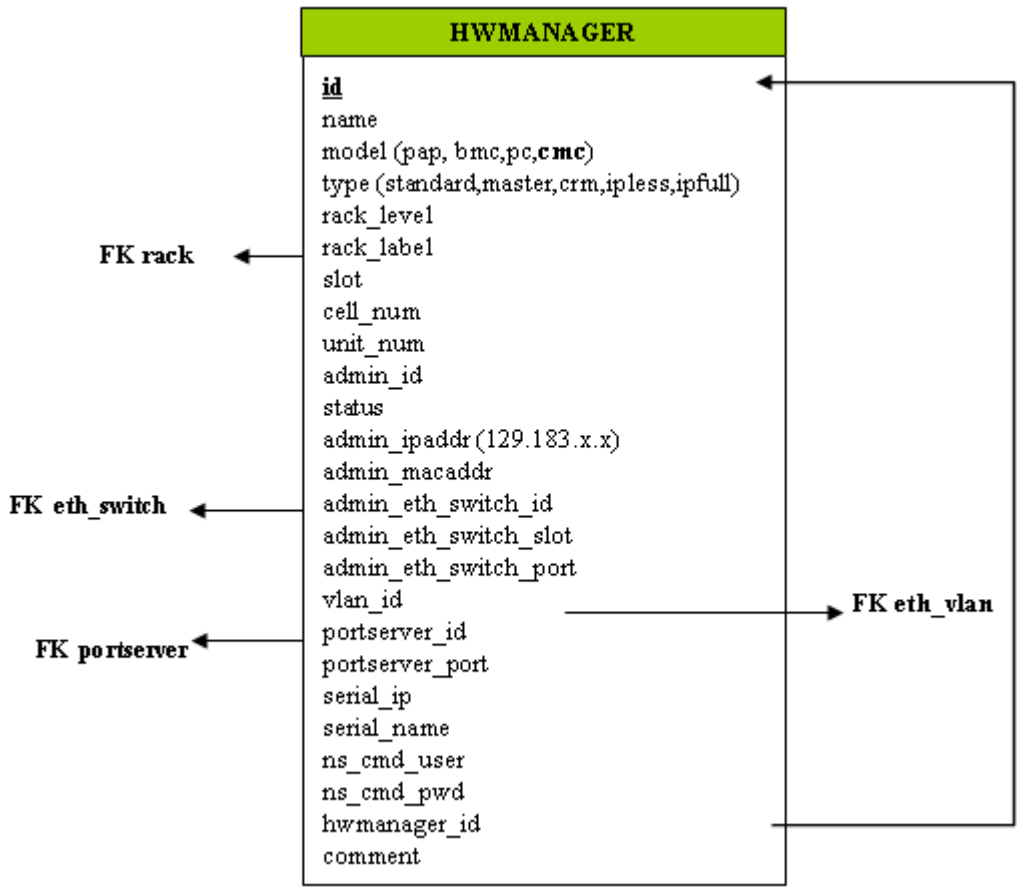
Figure 3-7. HWManager view
