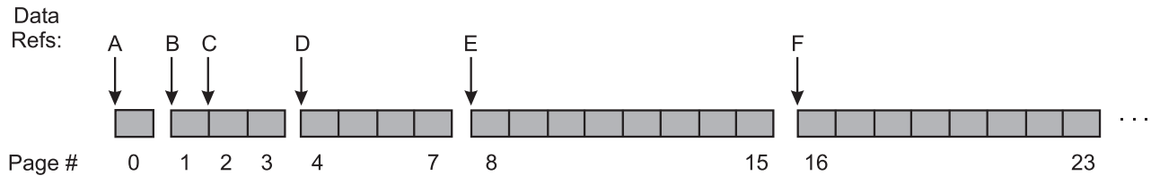
Figure 22. Sequential Read-Ahead Example. This illustration shows a row of blocks simulating a segmented track of file page numbers. These block segments are numbered 0, 1 through 3, 4 through 7, 8 through 15 and 16 through 23. The steps of a sequential read-ahead are found in the text immediately following the illustration.
