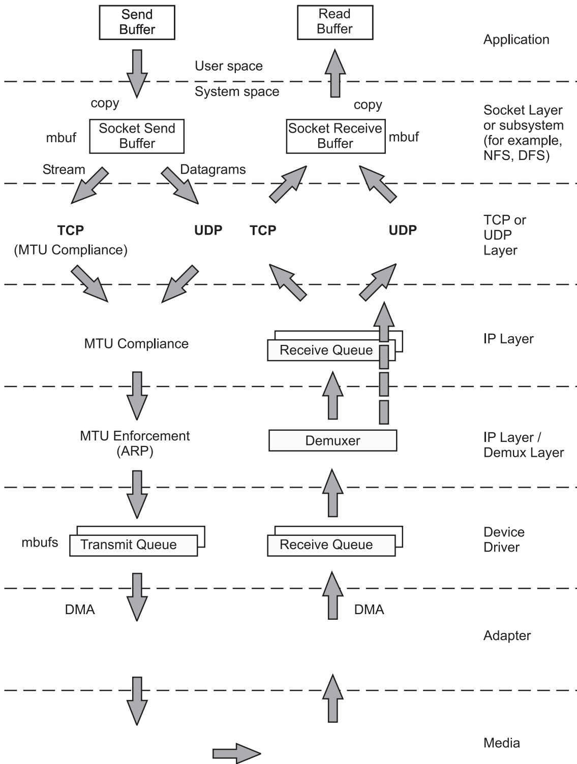
Figure 24. UDP and TCP/IP Data Flow. The figure shows the path of data from an application in one system to another application in a remote system. The steps of the data flow are described in the text immediately following the illustration.
