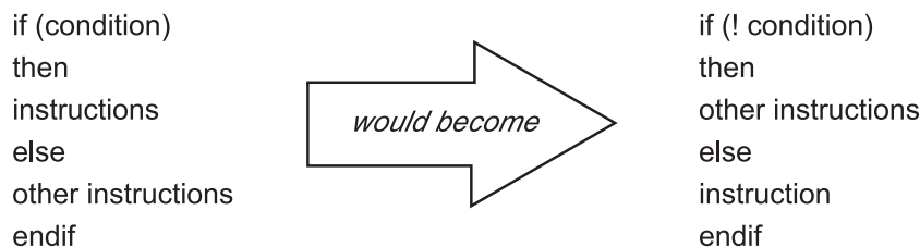
Figure 17. Example of Conditional Branch Recoding. The illustration shows how conditional branch recoding changes certain code. For example, the code If (condition) would become If (! condition) ; the code then stays then ; instructions becomes other instructions ; else stays else ; other instructions become instruction ; and endif stays endif .
