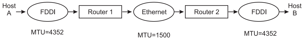
Figure 26. Inter-Subnet Fragmentation. This illustration shows a data path from Host A, through an FDDI with an MTU=4352, through Router 1, to the Ethernet with an MTU=1500. From there it goes to Router 2 and another FDDI with an MTU=4352 and out to Host B. An explanation of how fragmentation occurs in this example is described in the text immediately following the illustration.
