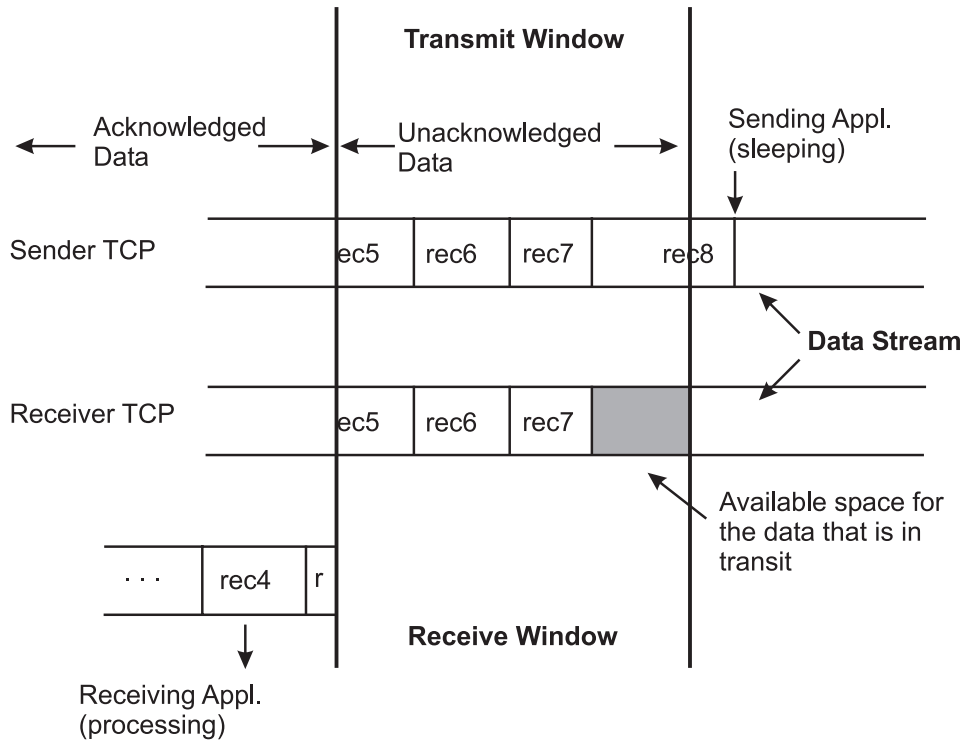
Figure 25. TCP Sliding Window. This illustration depicts the TCP Sliding Window. A full description is in the text immediately following the figure.
