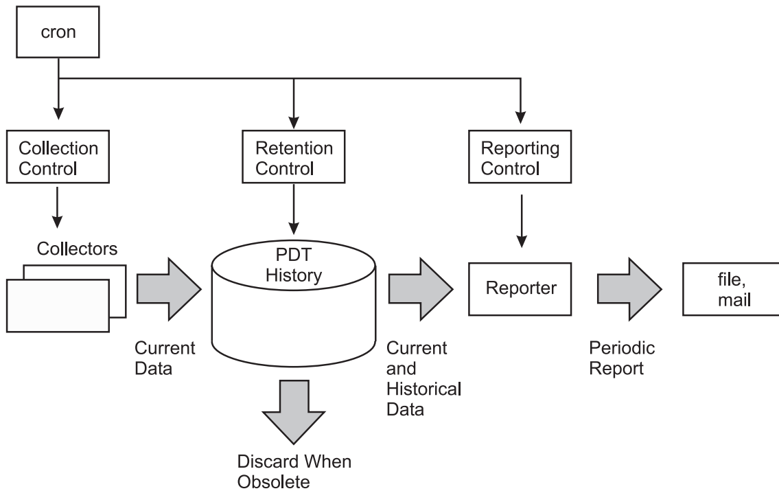
Figure 32. PDT Component Structure. This illustration is similar to an organizational chart with the three PDT application components at the top. They are; collection control, retention control and reporting control. A data path is drawn from collection control to collectors and then on to PDT History. A data path is drawn from retention control directly to PDT History. Data travels from Reporting control to the reporter and a periodic report is sent by file or mail. Data in PDT History can be discarded when it is obsolete or passed on to the reporter where periodic reports are sent by file or mail. All data is originated by the cron.
