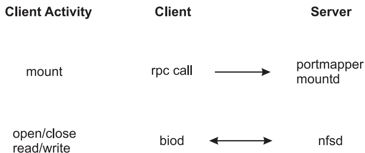
Figure 28. The Mount and NFS Process. This illustration is a three column table with Client Activity, Client, and Server as the three column headings. The first client activity is mount. An rpc call goes from the client to the server's portmapper mountd. The second client activity is open/close read/write. There is two-way interaction between the client's biod daemon and the server's nfsd daemon.
