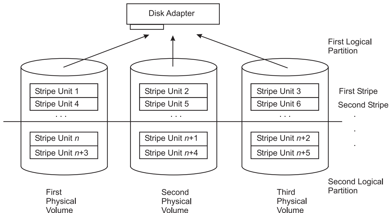
Figure 23. Striped Logical Volume /dev/lvs0. This illustration shows three physical volumes or drives. Each physical drive is partitioned into two logical volumes. The first partition, or logical volume, of drive 1 contains stripe unit 1 and 4. Partition 1 of drive 2 contains stripe unit 2 and 5 and partition 1 of drive 3 contains stripe unit 3 and 6. The second partition of drive one contains stripe unit n and n+3. The second partition of drive 2 contains stripe unit n+1 and n+4. Partition 2 of drive 3 contains stripe unit n+2 and n+5.
