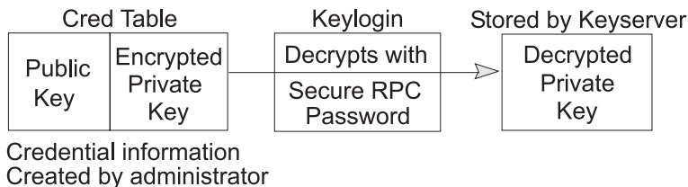
Figure 22. keylogin Generating a Principal's Private Key. This illustration shows cred table entries created by an administrator (the public key and the encrypted private key), which are decrypted by keylogin with the Secure RPC password, then stored by keyserver with the decrypted private key.
