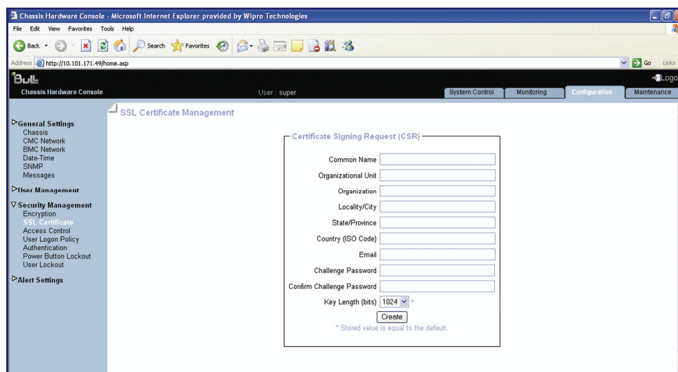
Figure 5-28. Page SSL Certificate Management (Gestion de certificat SSL)
