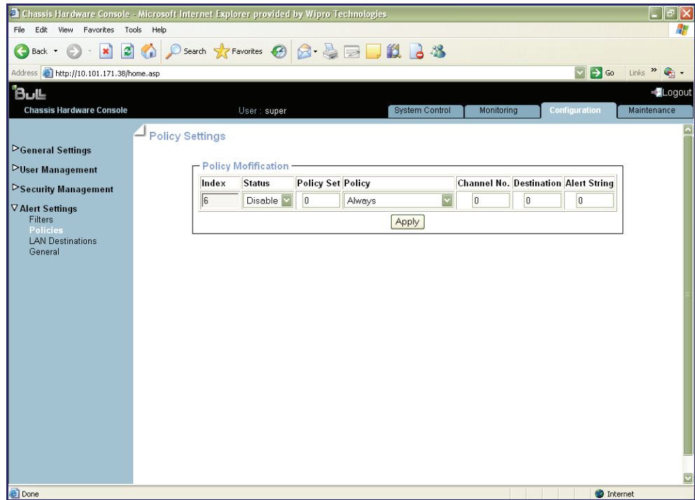
Figure 5-36. Page Policy Modification (Modification de politique)
