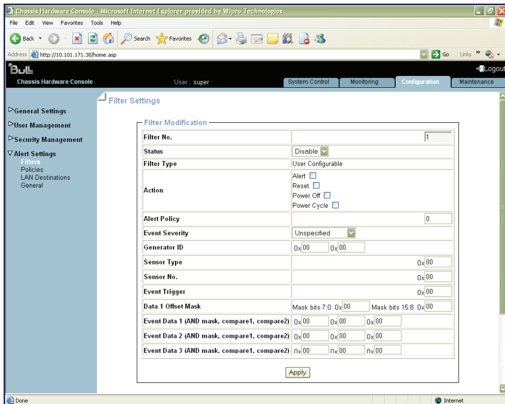
Figure 5-34. Page Filter Modification (Modification de filtre)
